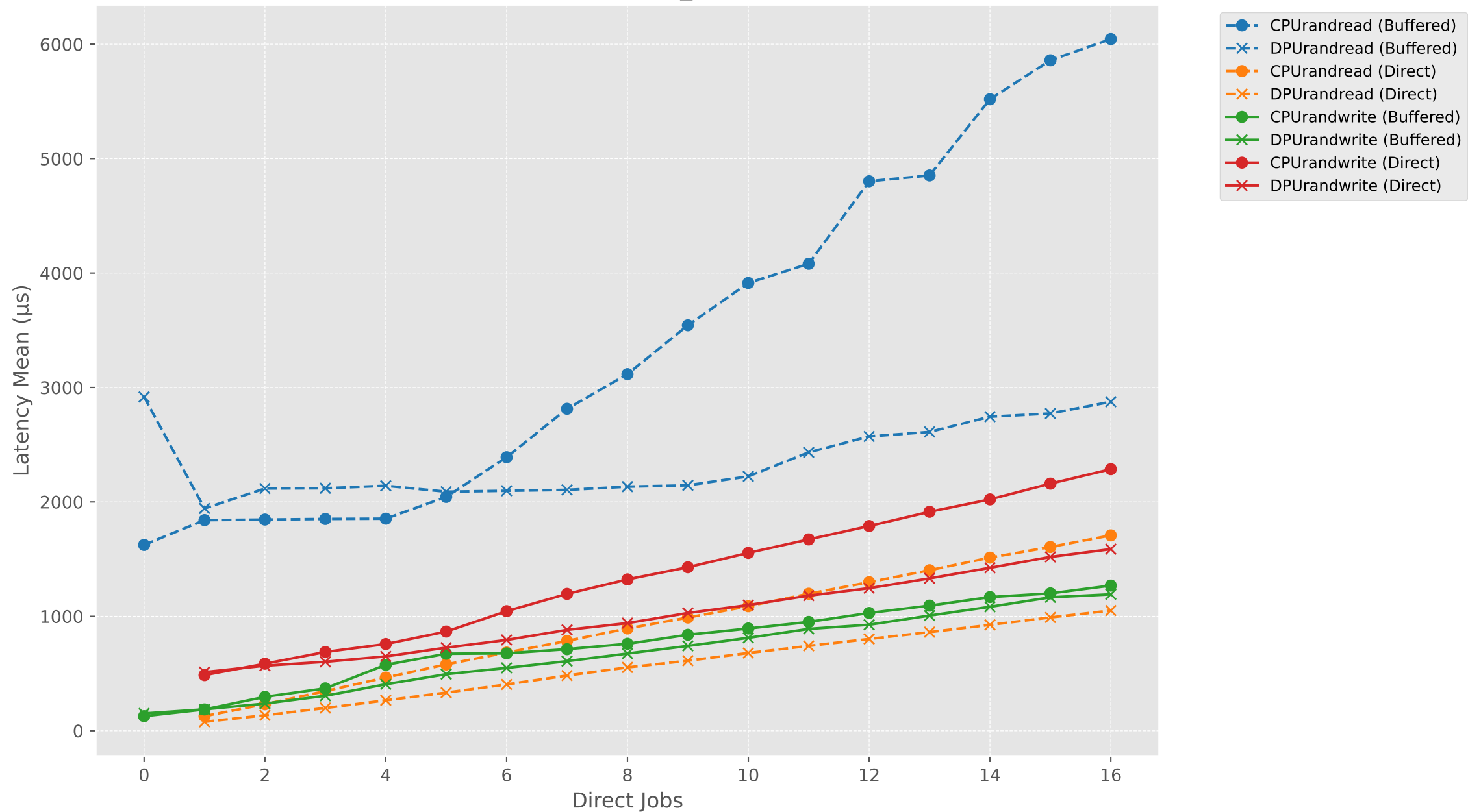
Latency Mean vs Direct Jobs (buffered1_directN) - RAND (CPU vs DPU)
